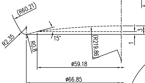
1 BOTTOM STACK PROFILE SCALE 2 : 1
